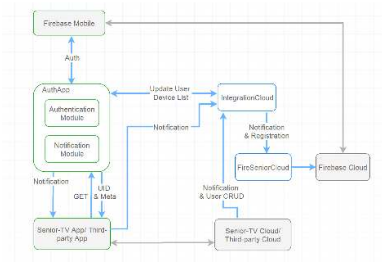
FIGURE 140. GENERAL ARCHITECTURE OVERVIEW
