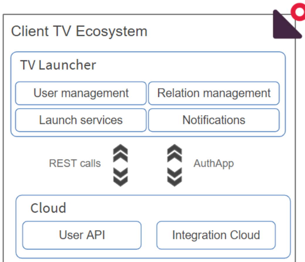
FIGURE 149. SENIOR-TV ECOSYSTEM ARCHITECTURE
