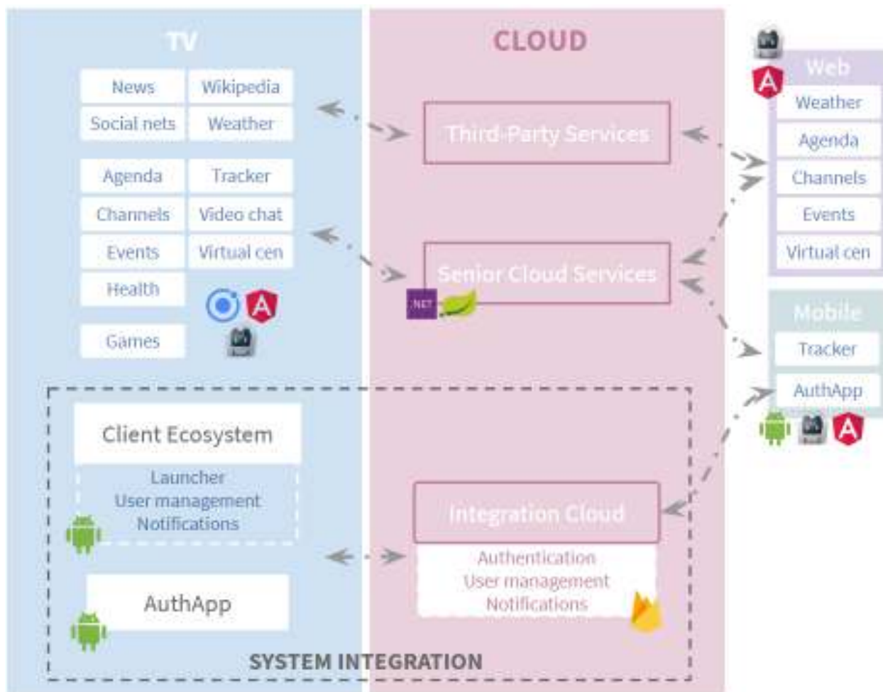
FIGURE 6. PLATFORM INTERACTION
