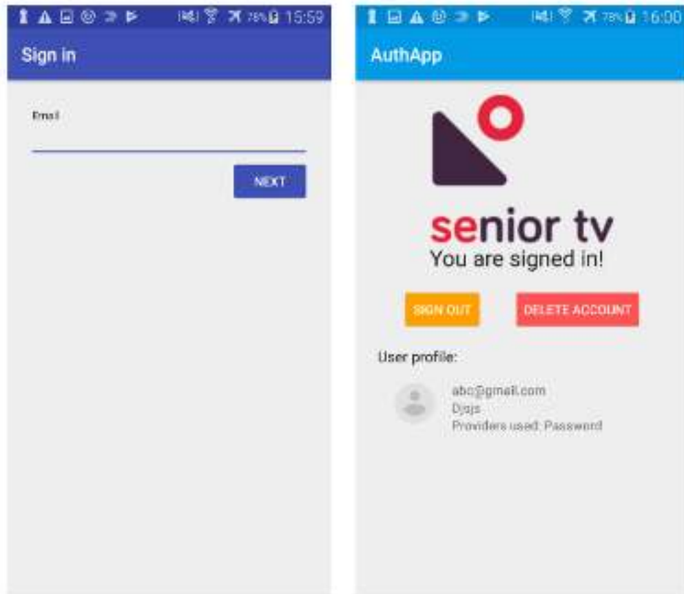
FIGURE 141. AUTHAPP SCREENS
