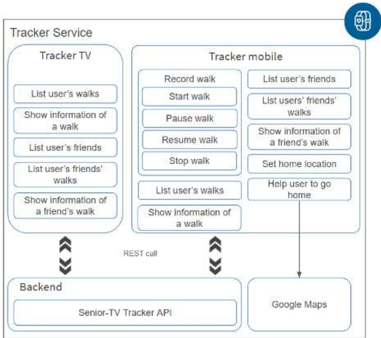
FIGURE 46. TRACKER ARCHITECTURE
