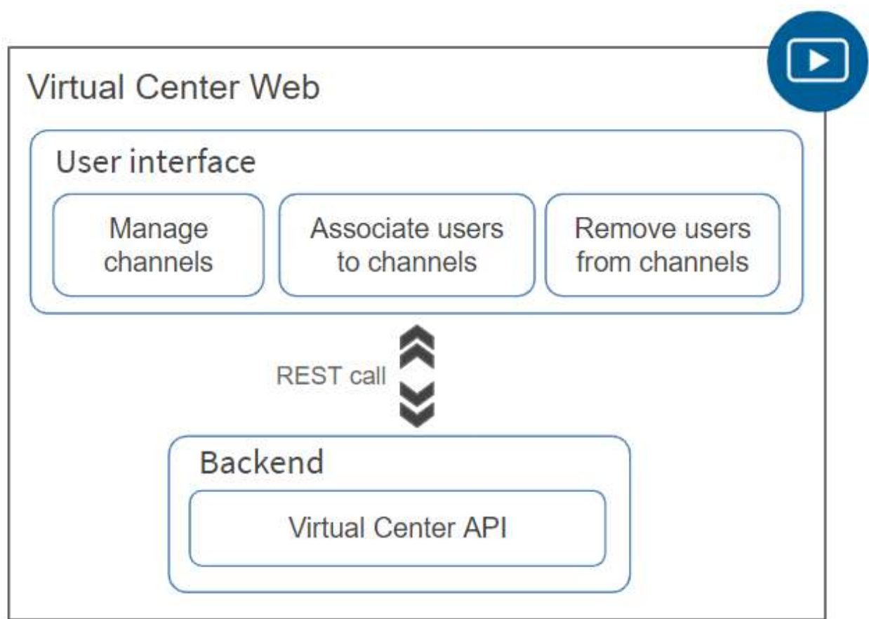
FIGURE 76. VIRTUAL CENTER WEB - ARCHITECTURE
