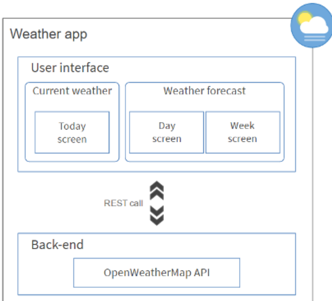
FIGURE 15. WHEATEAR APP ARCHITECTURE
