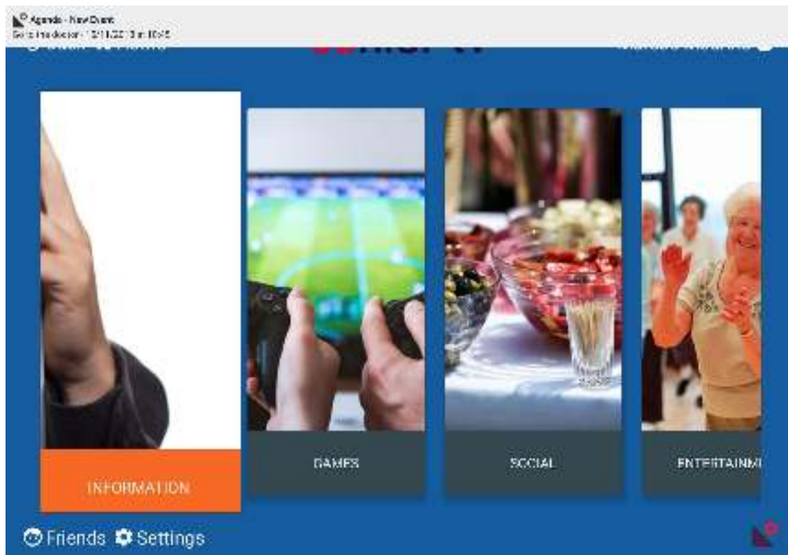
FIGURE 159. ECOSYSTEM - NOTIFICATION
