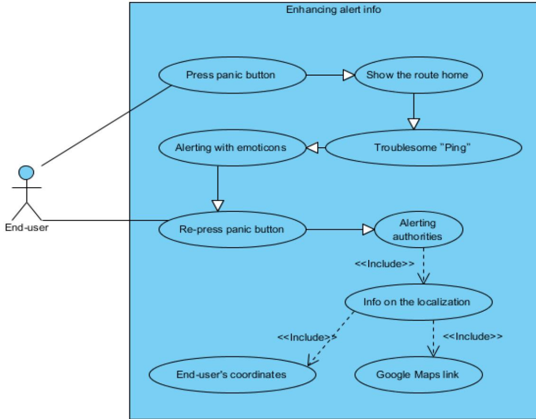
Figure 15. Use case diagram for the "Enhancing alert info" service
