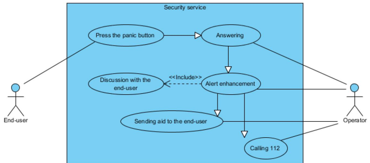
Figure 8. Use case diagram for the " Safety" Service
