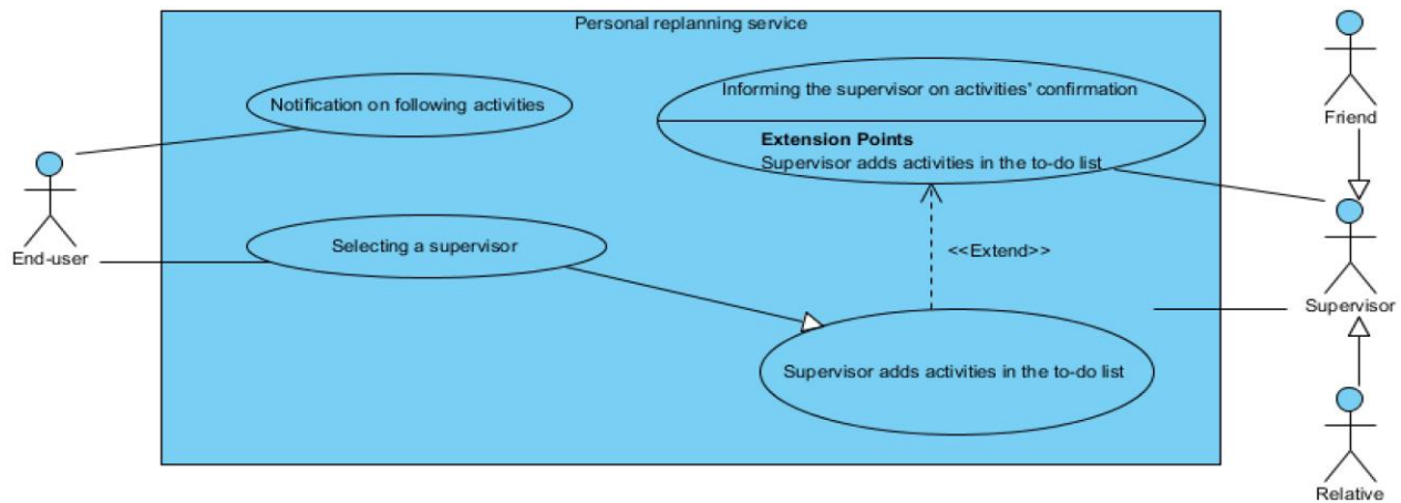
Figure 14. Use case diagram for the "Personal replanning" service
