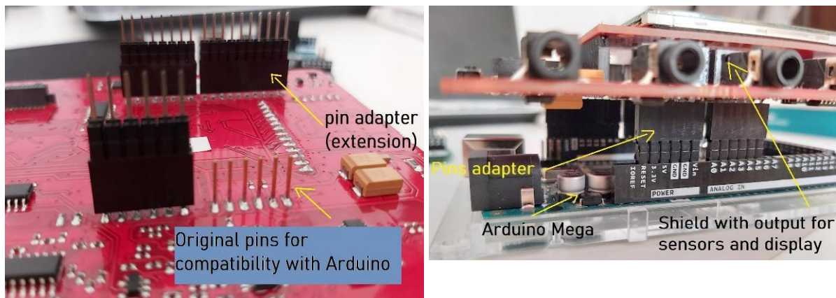
Figure 15 - Hardware adaptation by extending the required Arduino Mega pins
